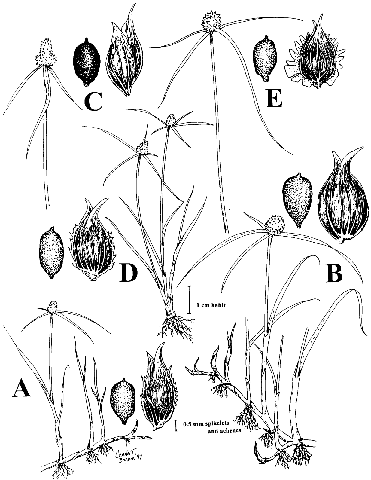
Figure 1. Achene, scale, and habit illustrations of Kyllinga species found in the continental United States: K. brevifolia —A; K. gracillima —B; K. odorata —C; K. pumila —D; and K. squamulata —E.
